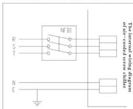
Wiring diagram of the single-compressor unit
